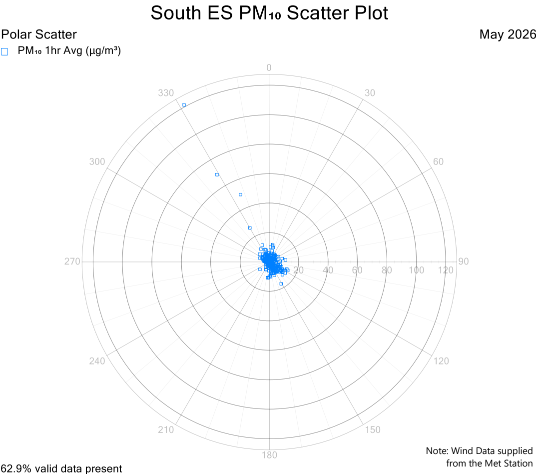
Figure 7: South E-Sampler PM 10 Scatter Plot 1-Hour Averages
