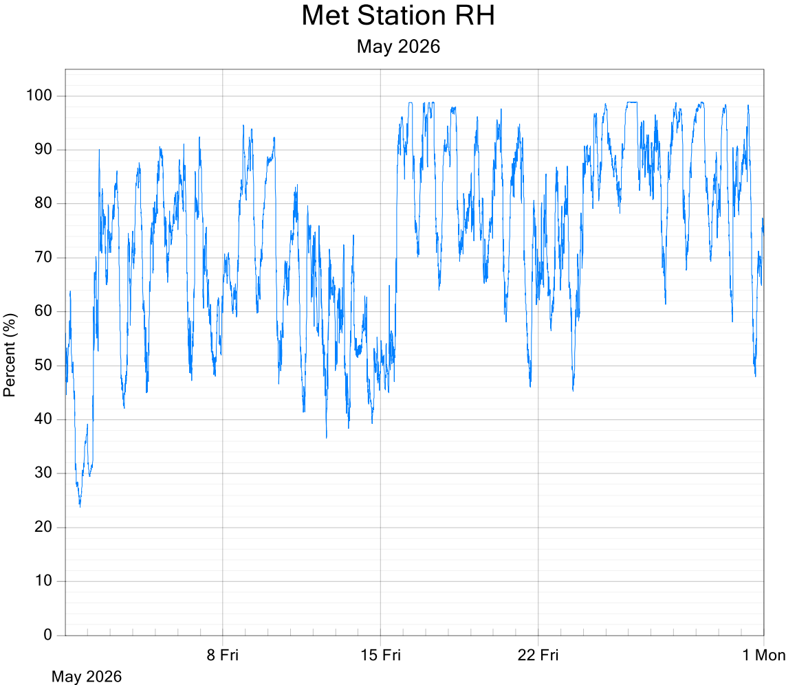
Figure 11: Met Station Relative Humidity 5-Minute Averages
