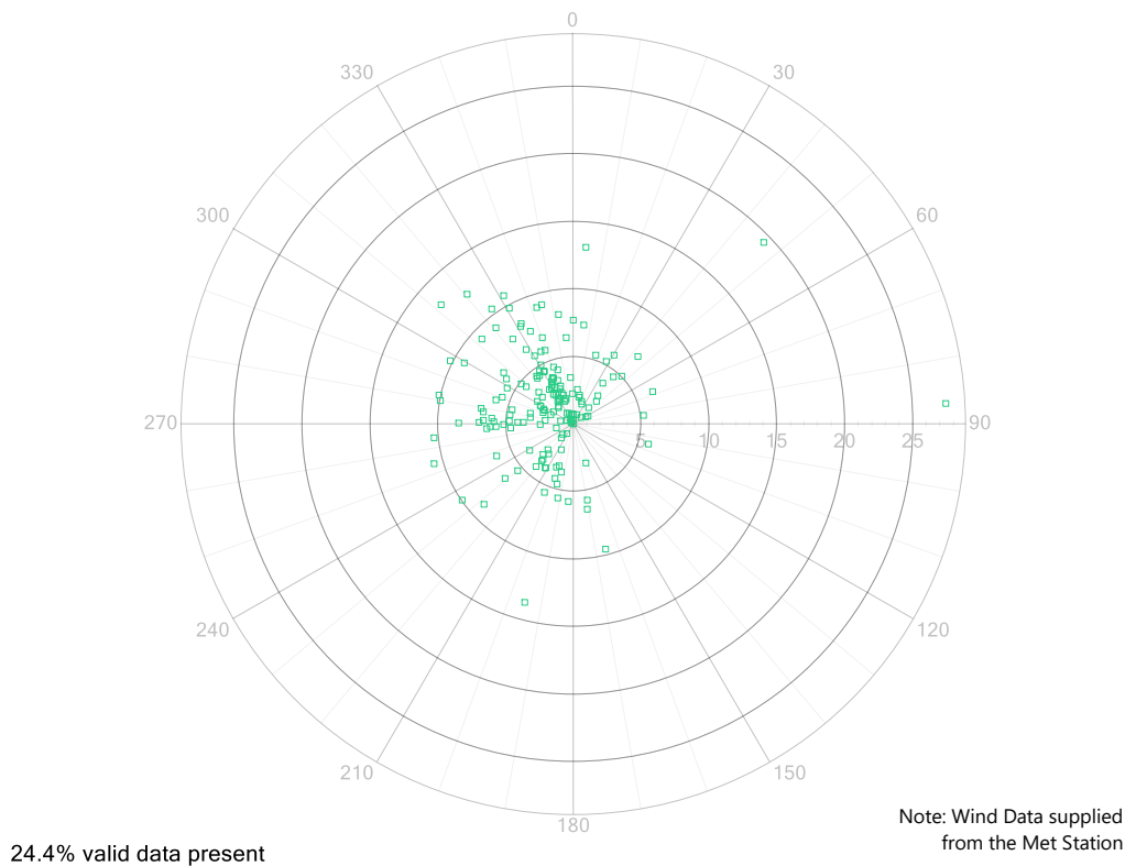
Figure 6: East E-Sampler PM 10 Scatter Plot 1-Hour Averages
