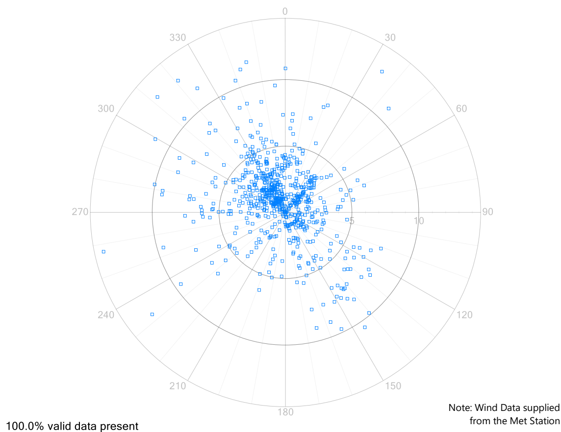
Figure 5: North E-Sampler PM 10 Scatter Plot 1-Hour Averages
