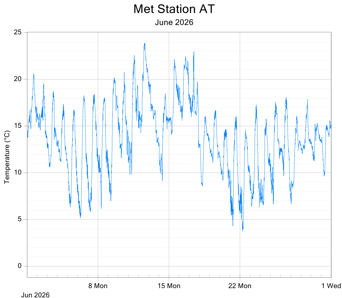
Figure 10: Met Station Ambient Temperature 5-Minute Averages
