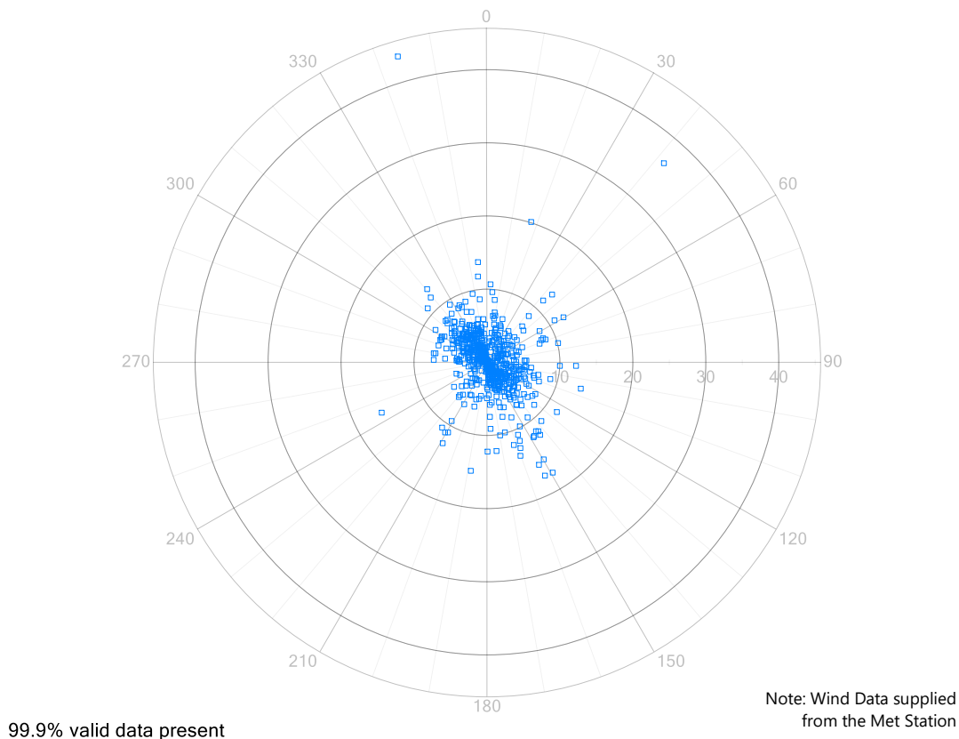
Figure 7: South E-Sampler PM 10 Scatter Plot 1-Hour Averages
