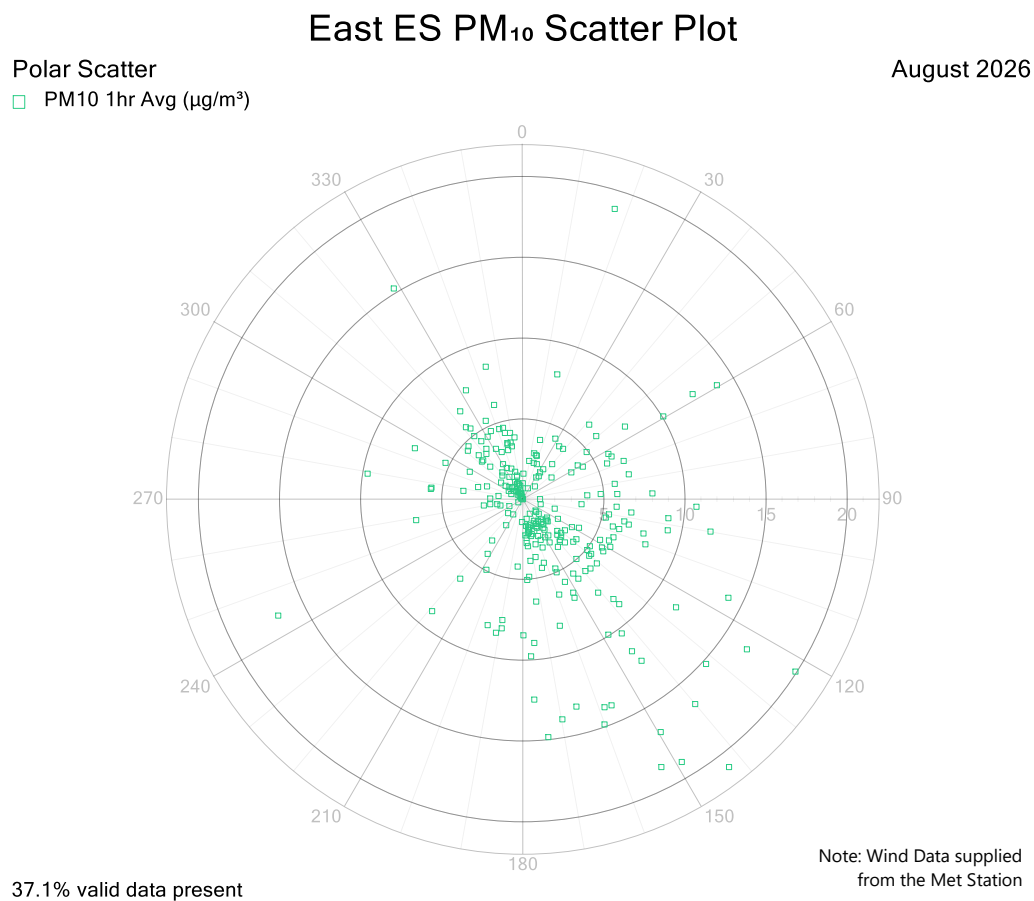
Figure 6: East E-Sampler PM 10 Scatter Plot 1-Hour Averages
